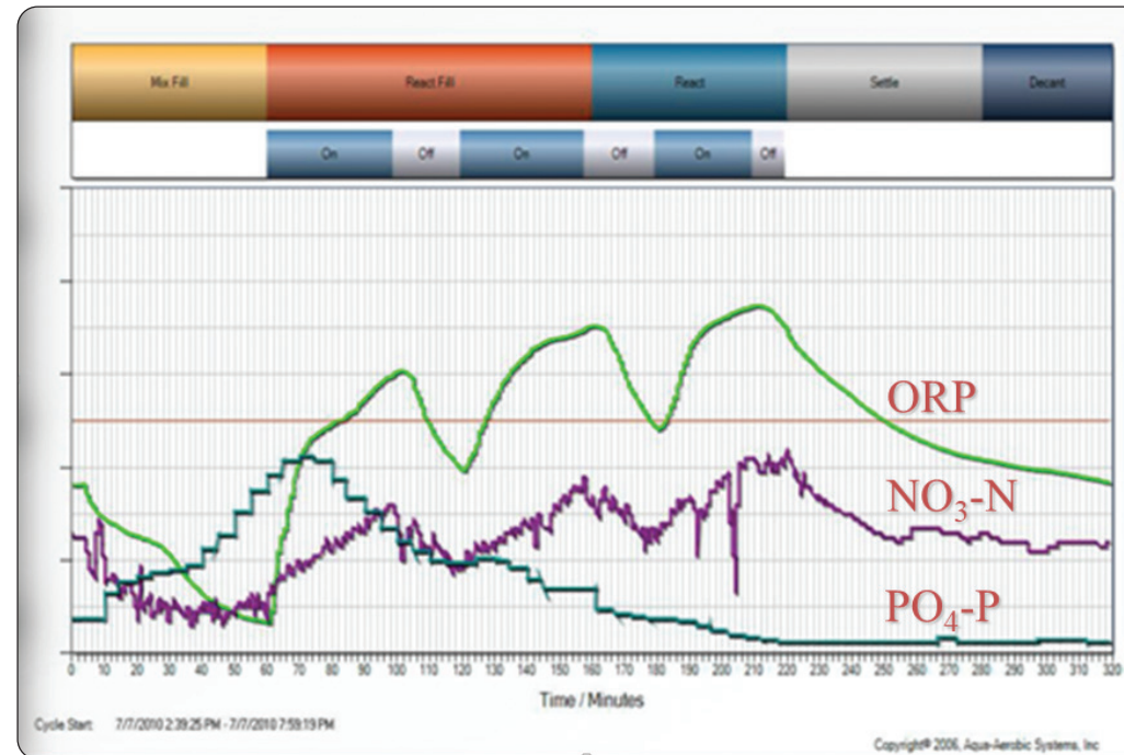
Nutrient profile allows for treatment optimization. The system can automatically adjust the environment and/or chemical addition to meet the required nutrient levels.
