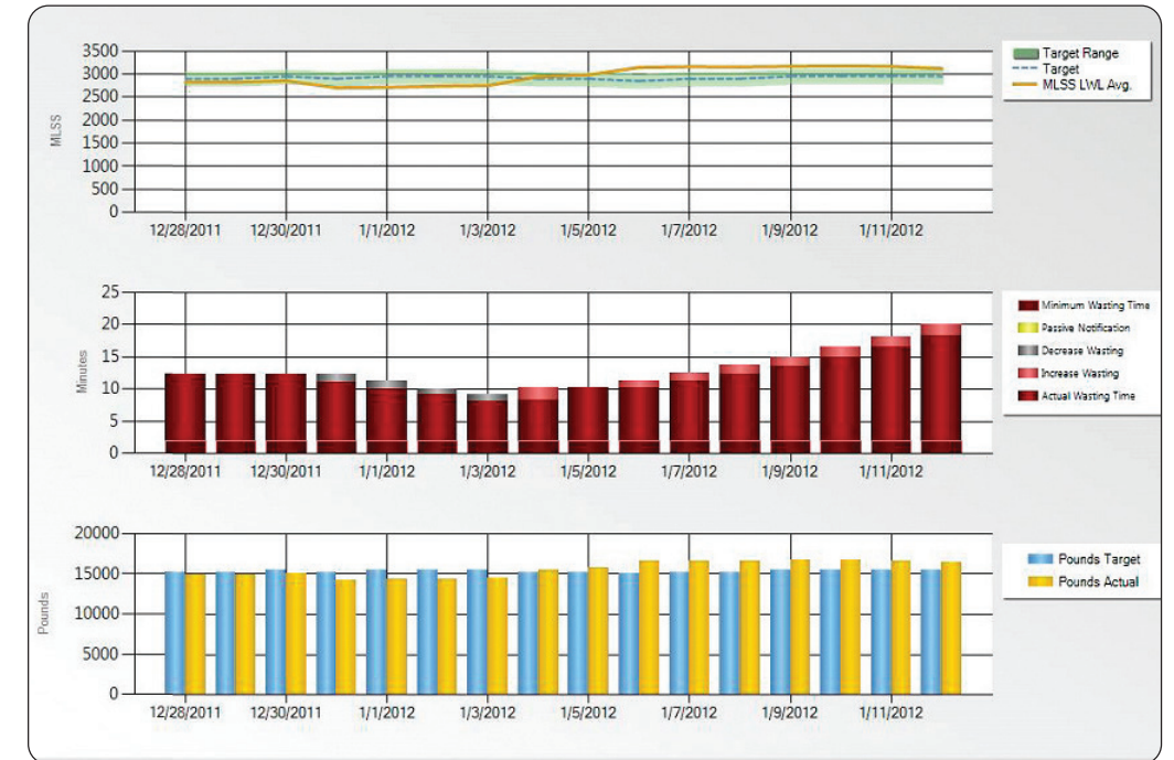
Active mass control creates a stable environment by automatically adjusting the wasting to the desired solids concentration. Operators are able to select a target MLSS, ideal F/M ratio or SRT.
