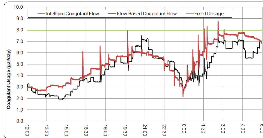
Ultra-low phosphorus can be efficiently achieved with the IntelliPro ® . The system adjusts the chemical to the influent loading to avoid overdosing while ensuring the effluent is met.
