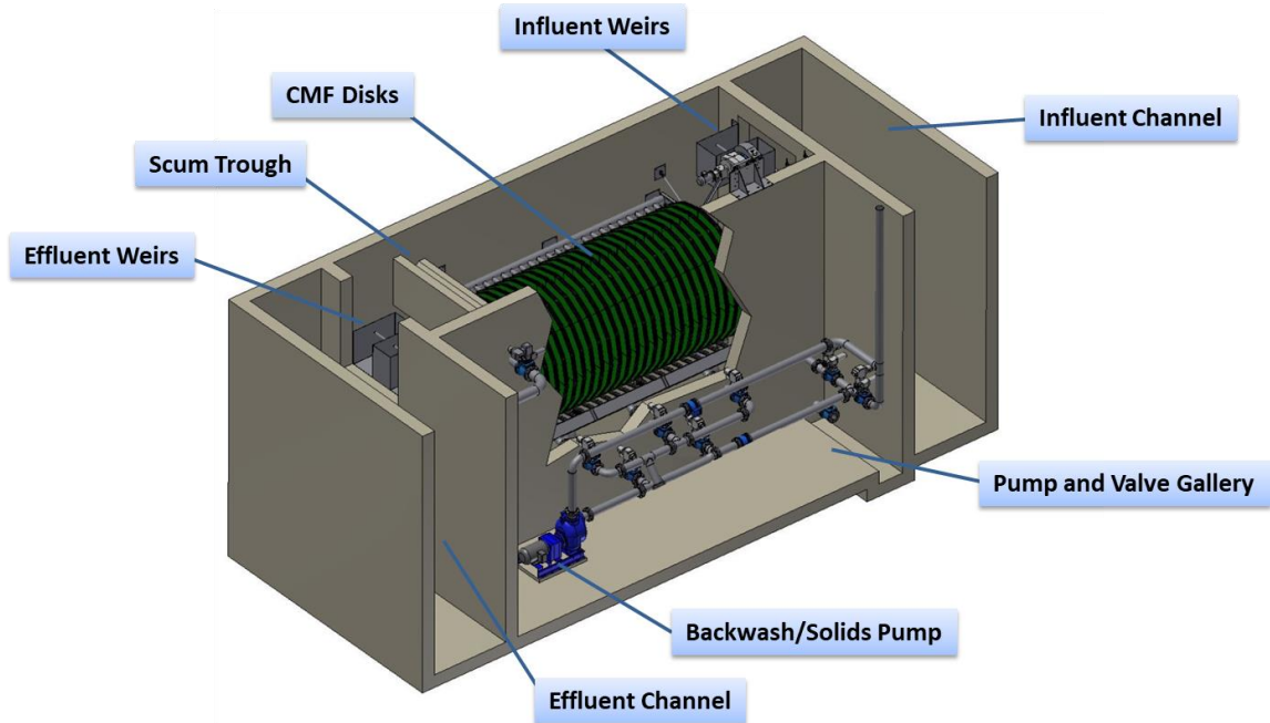
Figure 8: AquaStorm® Concrete Unit – 108 ft² Disks
