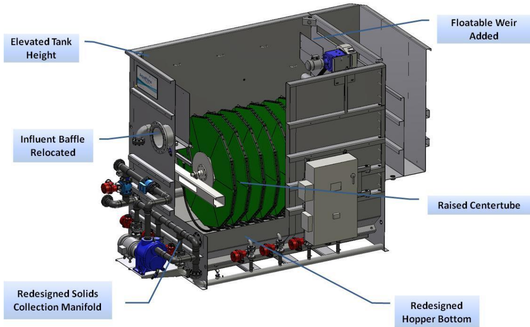
Figure 9: AquaStorm® Package Unit – 54 ft² Disks
